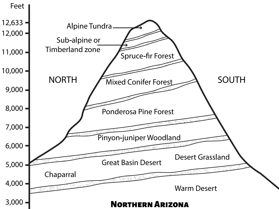
Figure 2. Life Zones of Northern Arizona based on elevation and aspect (northern aspects are generally cooler/wetter and southern warmer/drier). Life Zones are grouped based on dominant vegetation types; however, many minor species will follow these same zones.
